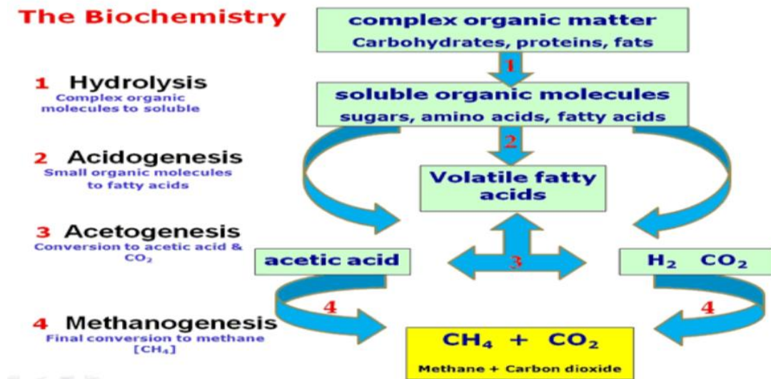
Fig. 1: Anaerobic digestion degradation steps
