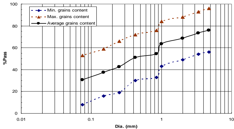
Fig. 3: Maximum, minimum and average grain size distribution curves of soil in Wadi Arar
