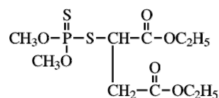
Fig. 1: Structural formula of Malathion
