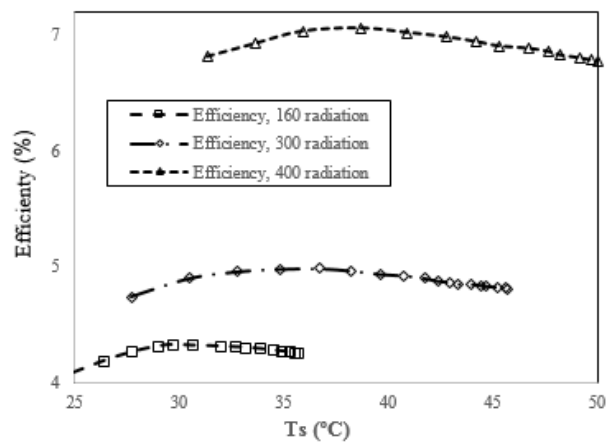
Fig. 7: Effects of surface temperature on efficiency under different radiation
