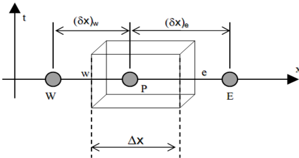
Fig.3: Grid system of an unsteady one-dimensional computational domain
